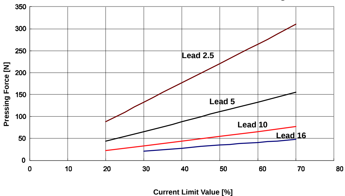
RA4C/R Current Limit Value and Pressing Force
