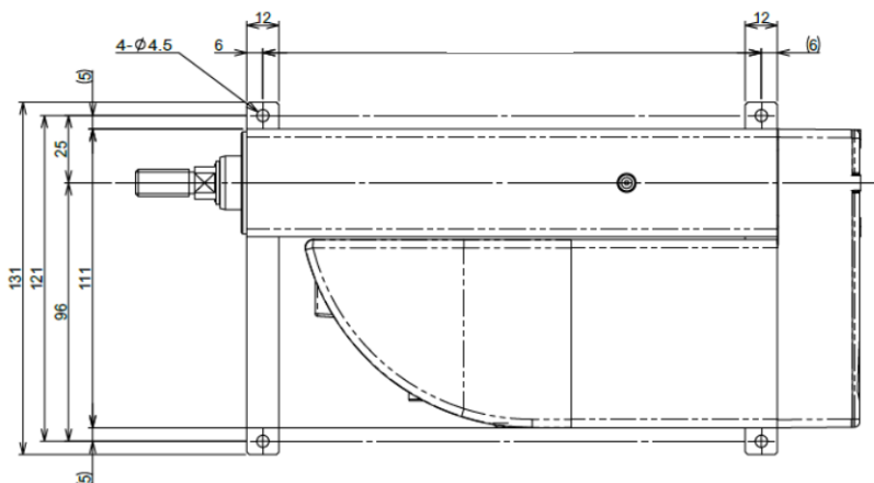
RCP6S-RA4R Motor Left Side-Mounted (ML), Motor Right Side-Mounted (MR)
