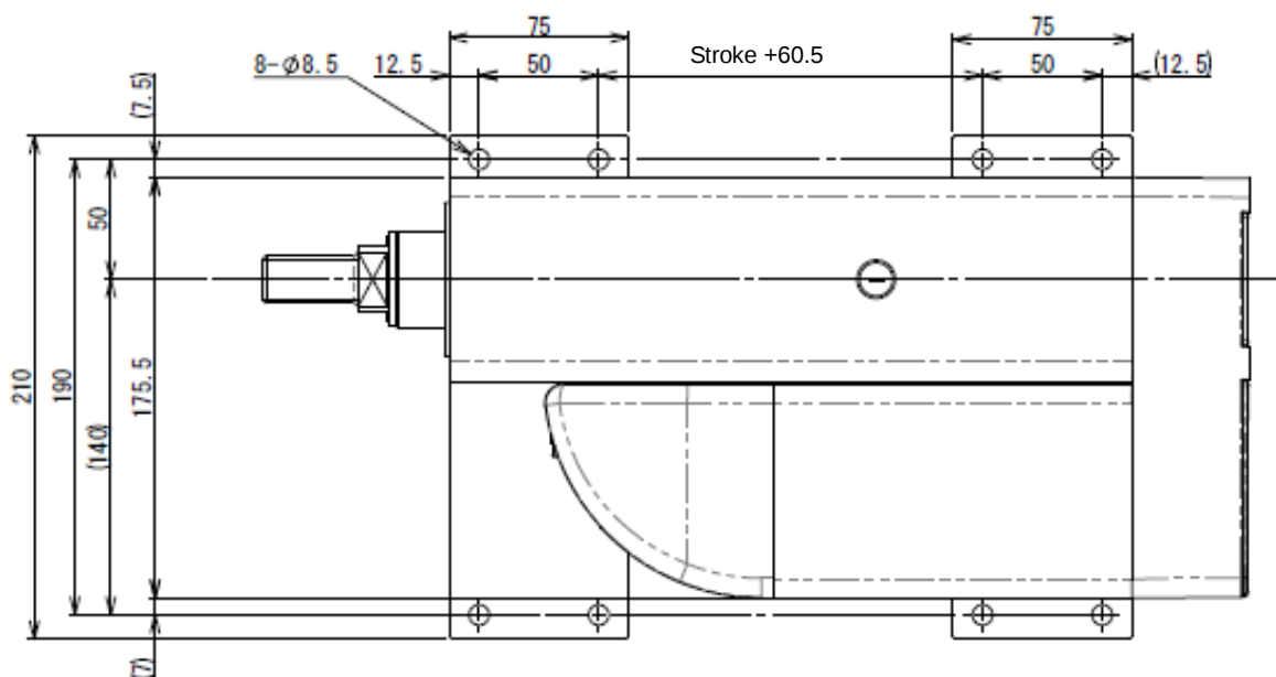
RCP6(S)-RA8R Motor Left Side-Mounted (ML), Motor Right Side-Mounted (MR)
