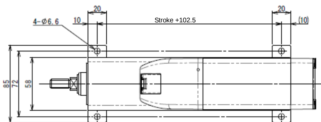
RCP6(S)-RA6R Motor Top Side-Mounted Type (Model: MT)
