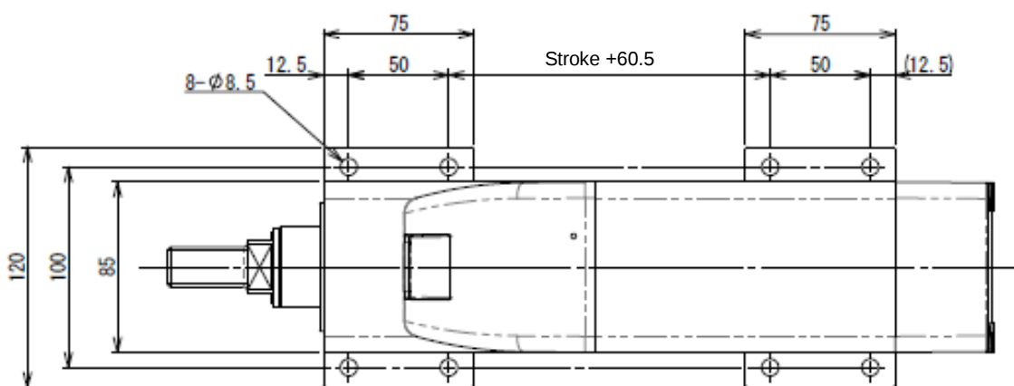
RCP6(S)-RA8R Motor Top Side-Mounted Type (Model: MT)
