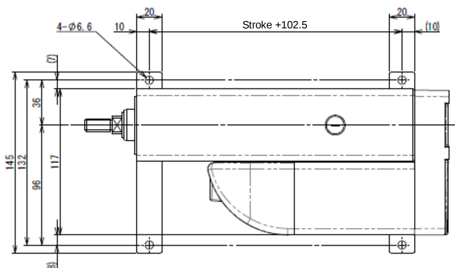
RCP6(S)-RA6R Motor Left Side-Mounted (ML), Motor Right Side-Mounted (MR)
