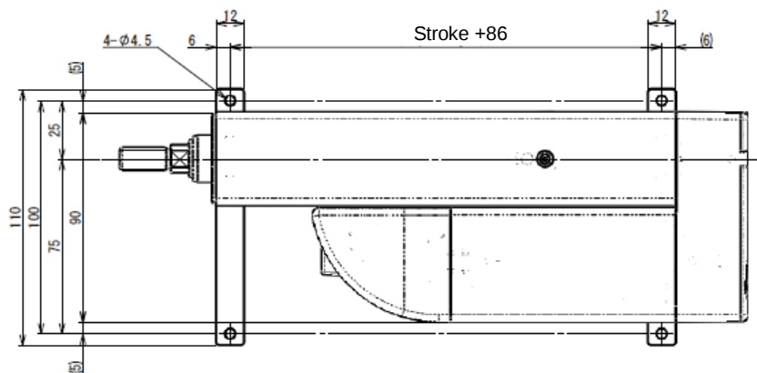
RCP6-RA4R Motor Left Side-Mounted (ML), Motor Right Side-Mounted (MR)
