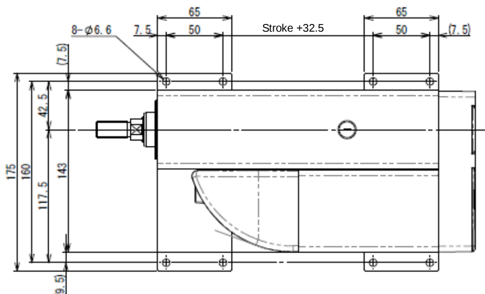
RCP6(S)-RA7R Motor Left Side-Mounted (ML), Motor Right Side-Mounted (MR)
