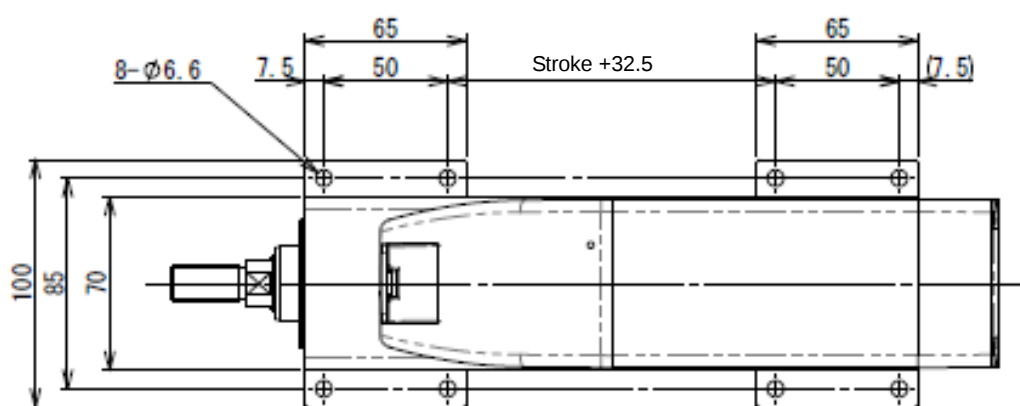
RCP6(S)-RA7R-MT Motor Top Side-Mounted Type (Model: MT)
