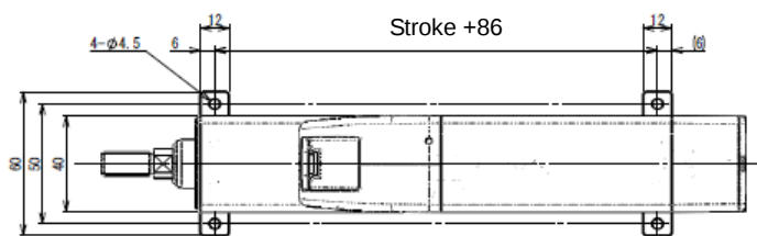
RCP6(S)-RA4R Motor Top Side-Mounted Type (Model: MT)
