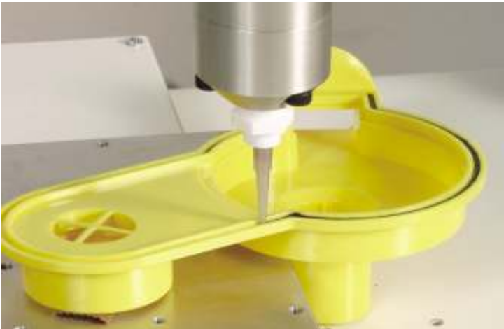
▲ TS941 - gasketing.
