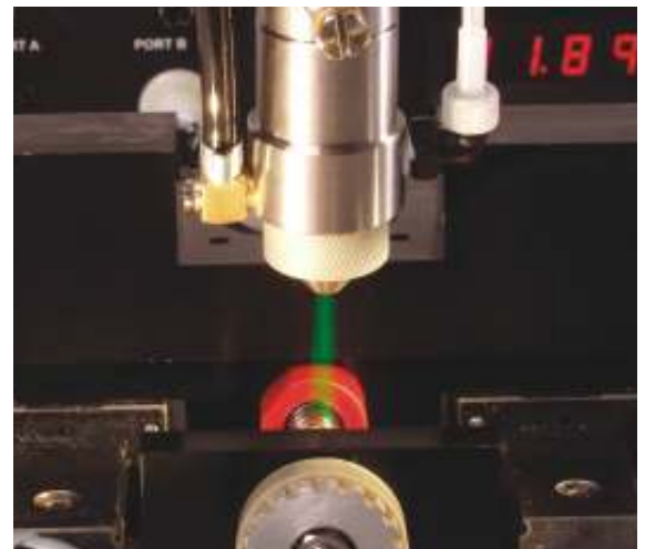
TS5540 Spray Valve - spray lubricant on feed screw. ►
