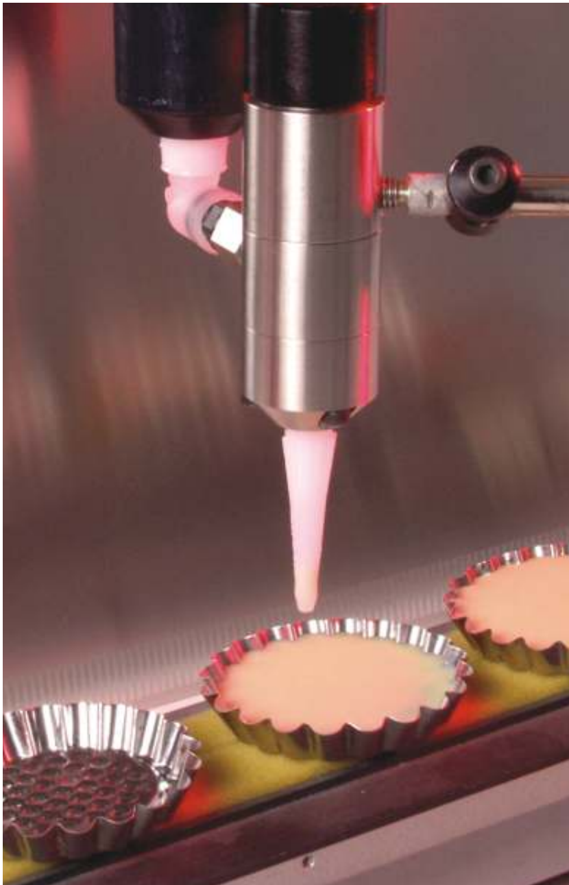
▲ TS941 - high-speed filling.
